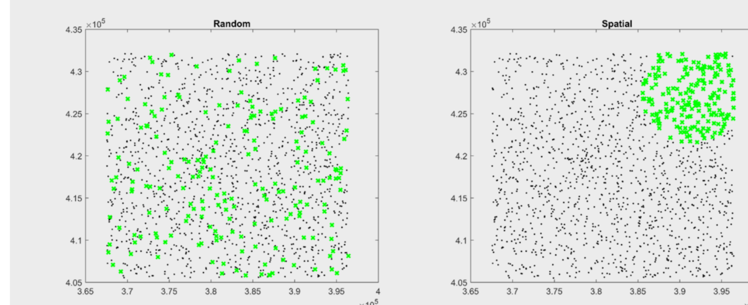
Fig. 3 Random and spatial point sampling.
