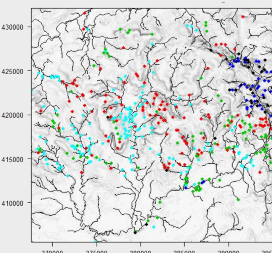
Fig. 6 Results of the cluster analysis using k-means on the verified records. Location was not incorporated into the clustering algorithm but is used here to display the cluster pattern.
